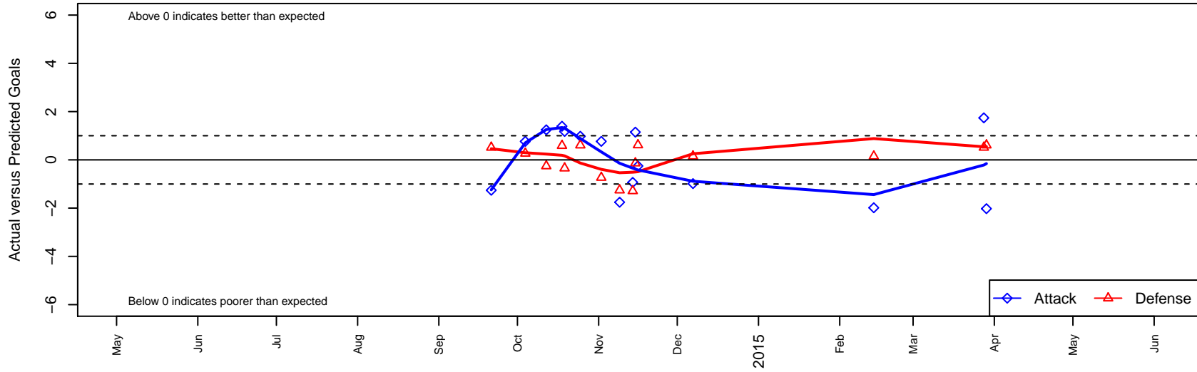
San Juan SC ECNL G00 Dots are actual minus expected GF (blue circles) and GA (red triangles). Blue line is smoothed change in attack strength. Red is smoothed change in defense strength.
